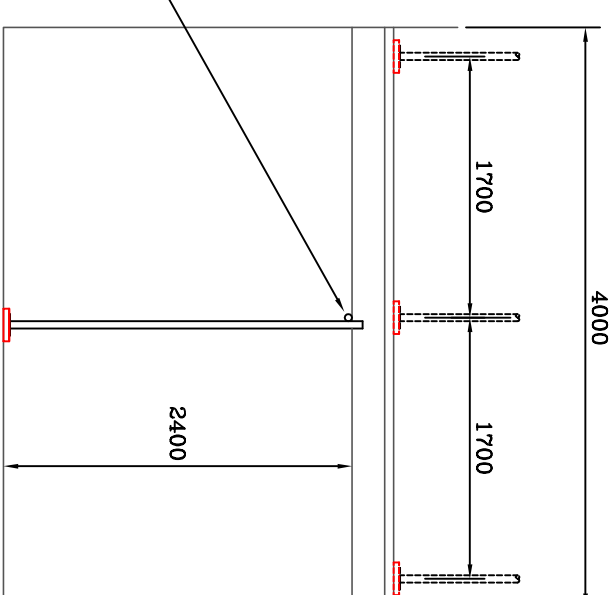
SECTION B-B
