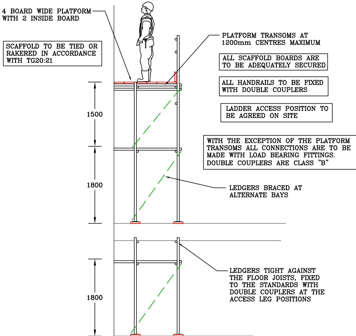
TYPICAL SECTION AT 2.0M CENTRES.
